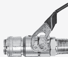
Disconnection with Purge Plug.
