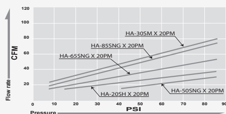
PRESSURE - FLOW RATE
